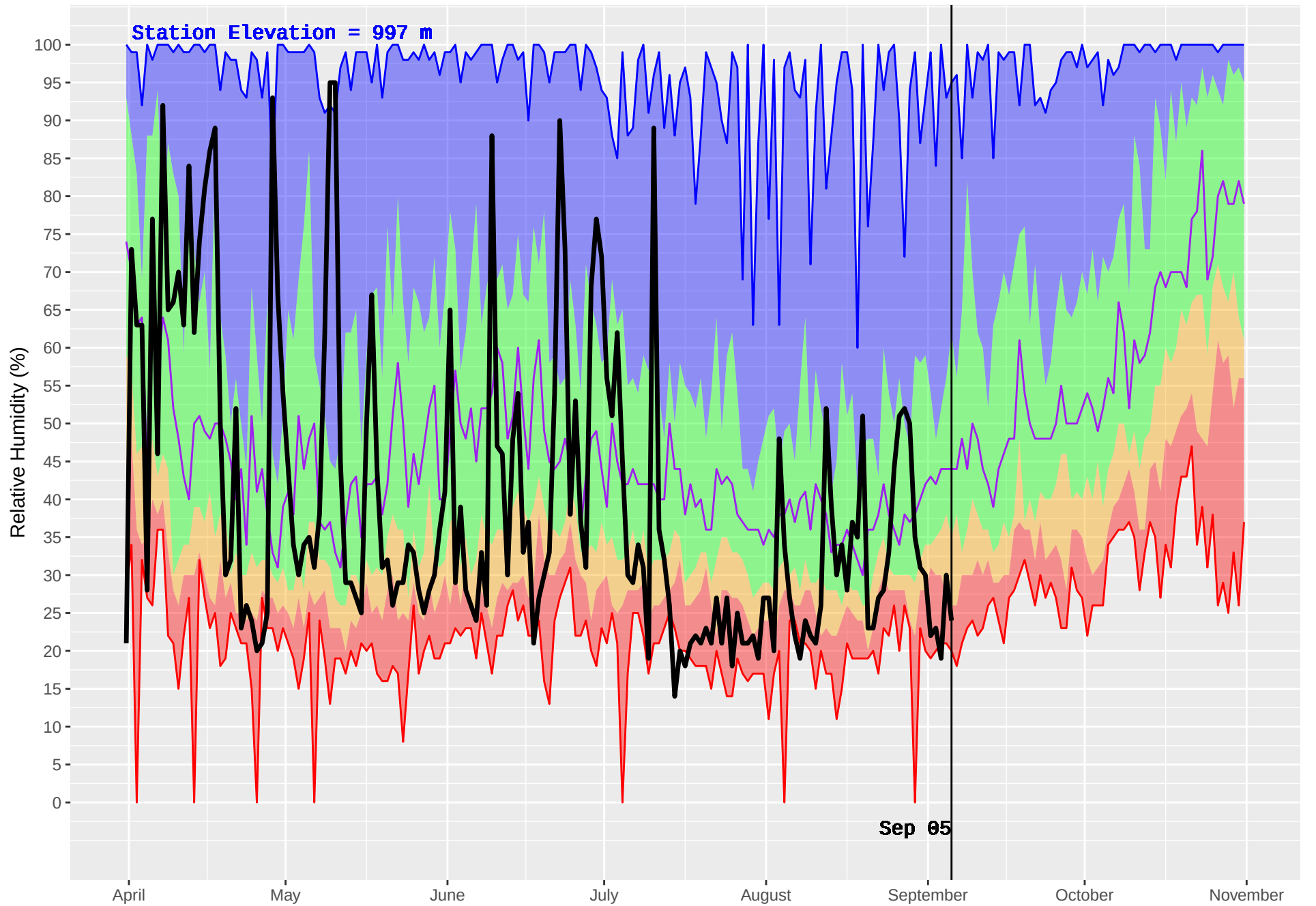
SMALLWOOD (404) : Historical (1991–2016) and Current (2018) Daily Relative Humidity
