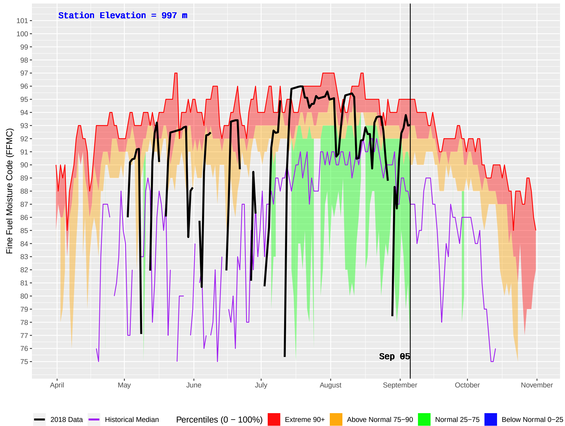
SMALLWOOD (404) : Historical (1991–2016) and Current (2018) Daily Fine Fuel Moisture Code (FFMC)
