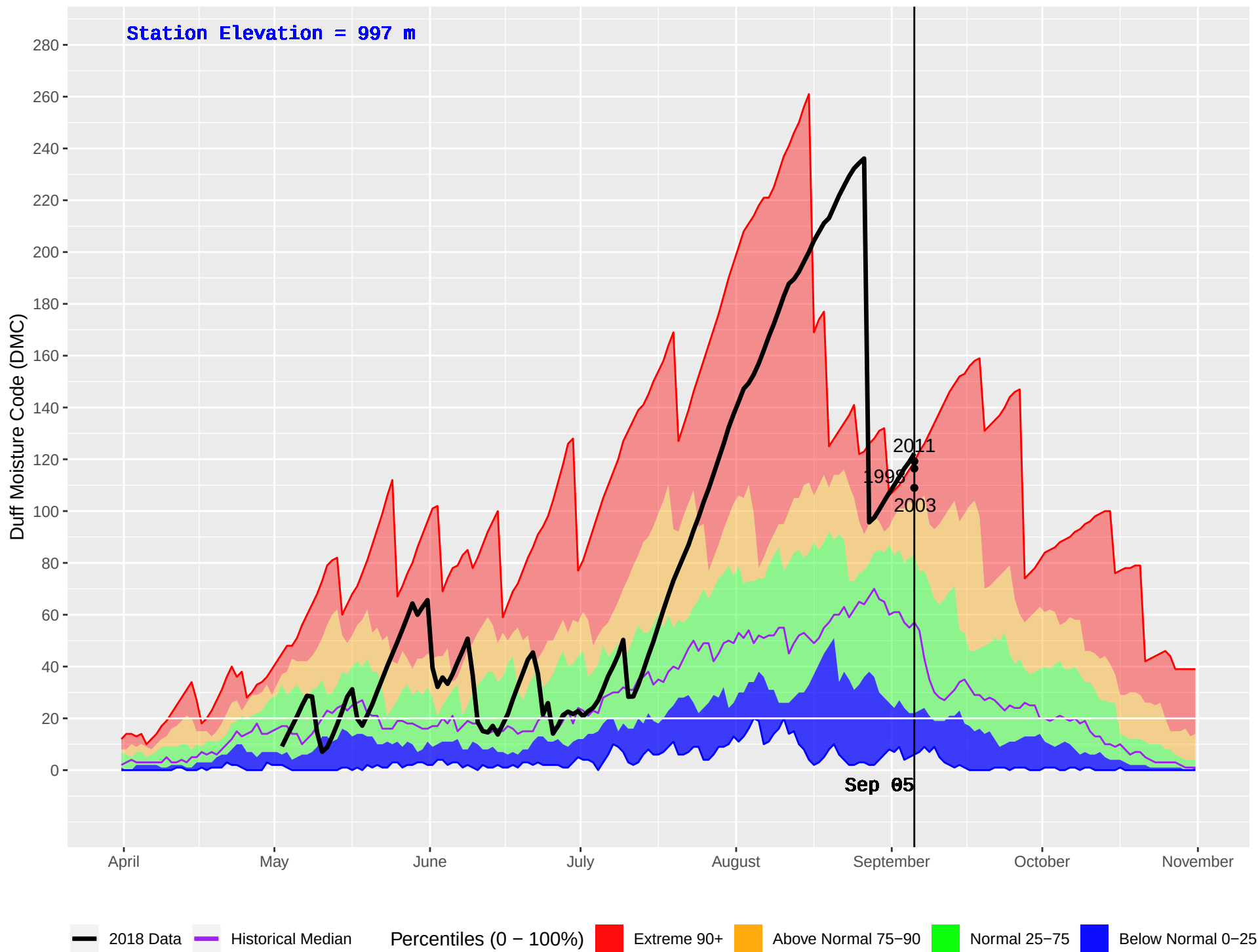
SMALLWOOD (404) : Historical (1991–2016) and Current (2018) Daily Duff Moisture Code (DMC)
