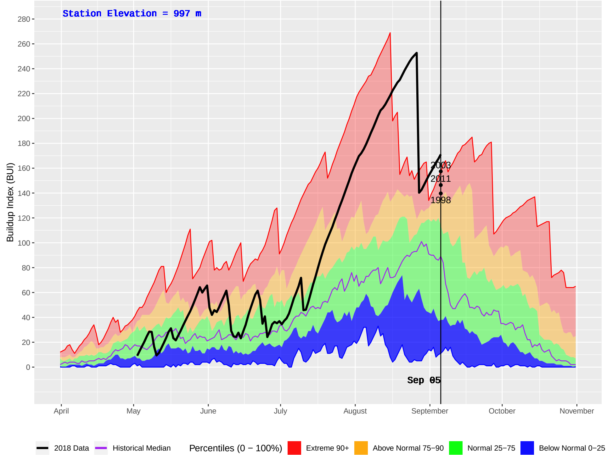
SMALLWOOD (404) : Historical (1991–2016) and Current (2018) Daily Buildup Index (BUI)
